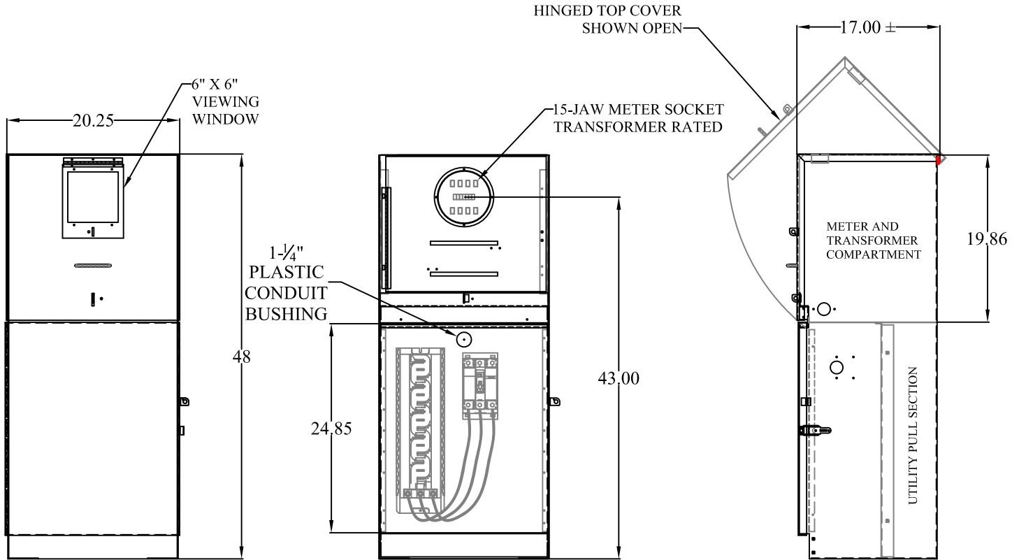
FRONT VIEW
